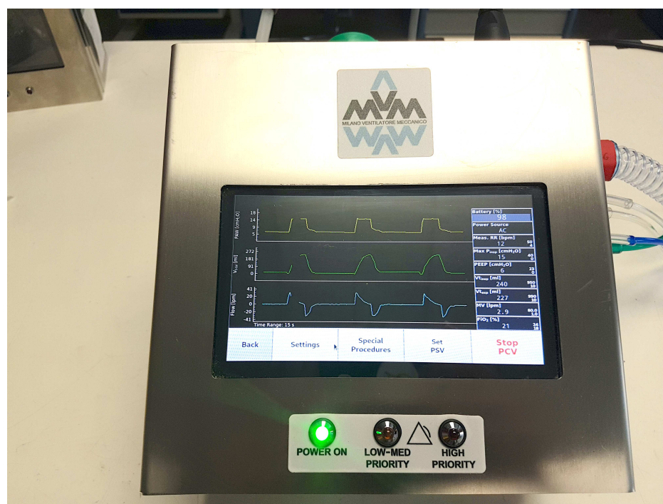
FIG. 4: Front view of the MVM.
